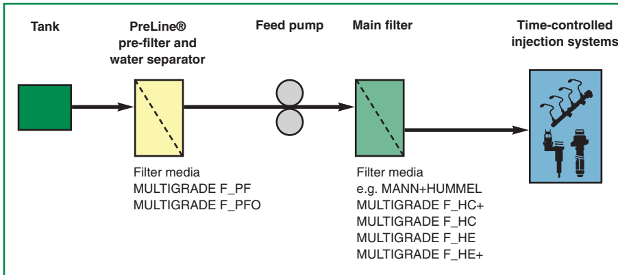
Integration of PreLine® into the fuel system of a commercial vehicle
